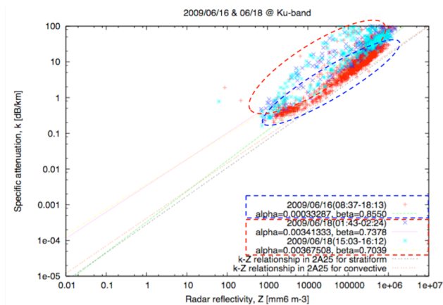
Figure 8. The k - Z relationship for Ku-band that is estimated by the 400MHz-WPR depending on rain type (weak and strong rain)
