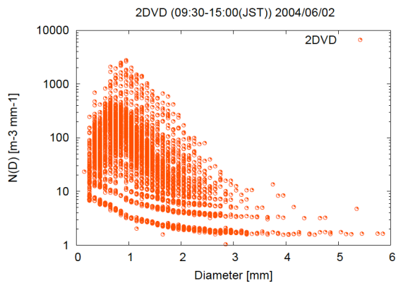
Figure 6. Raindrop size distribution observed by the 2DVD, 2004/06/02, 09:30-15:00 (JST)
