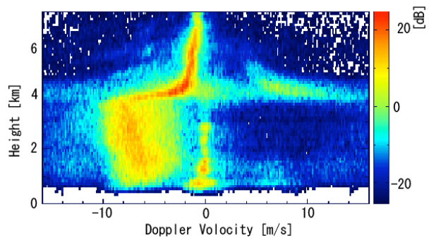
Figure 2. Doppler spectrum observed by the 400-MHz WPR
