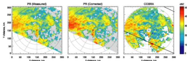
Figure 4. Comparison of horizontal radar reflectivity distribution for the PR and COBRA at a height of 2km (2004/06/09)
