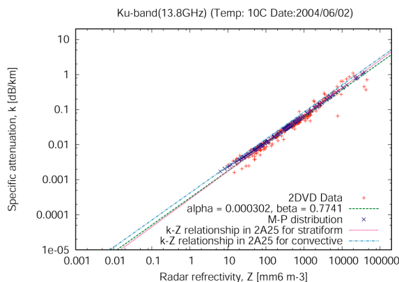
Figure 7. The k - Z relationship for Ku-band estimated by use of the 2DVD
